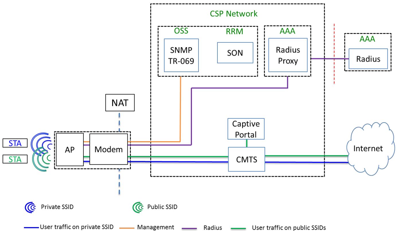
Figure 3.6 IPv4 Tunnels architecture
