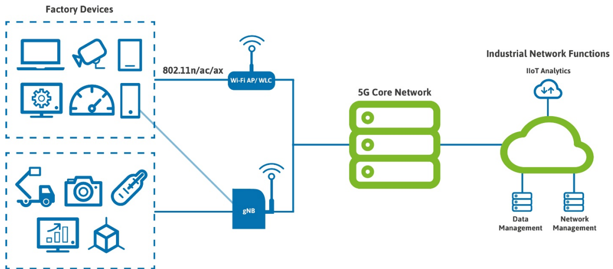
Figure 3-2. Example deployment of the Factory of the Future using 5G and Wi-Fi
