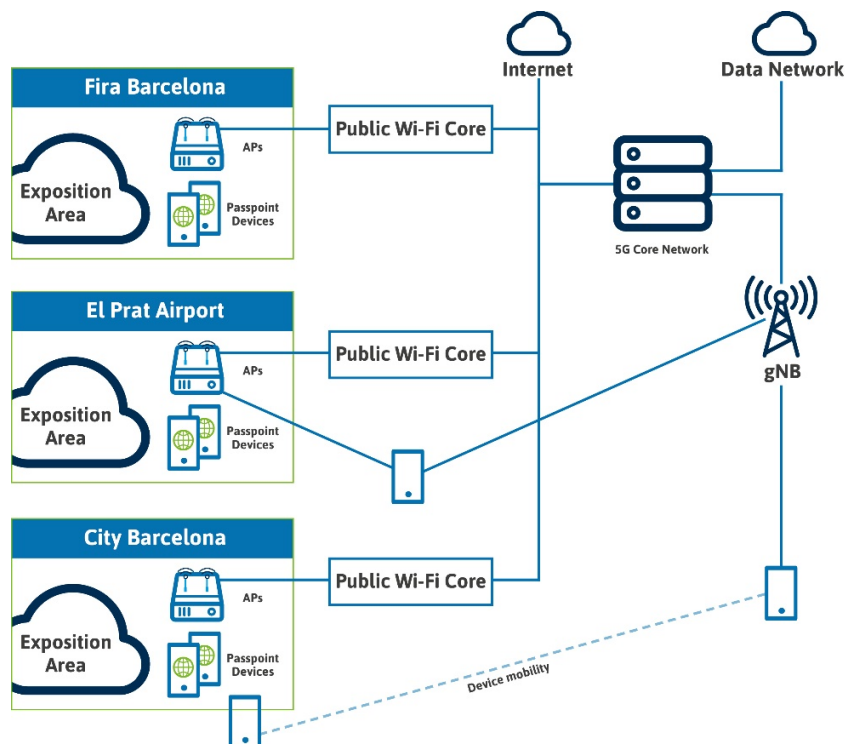
Figure 3-4 Example Deployment for Convergence of Public Wi-Fi with 5G
